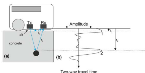
Figure 1. Layout of a survey on a reinforced concrete structure using a ground-coupled GPR system, b corresponding GPR signal output
