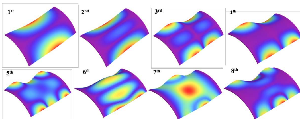
Figure 3. The open circular cylinder. Mode shapes of the lowest eight modes.
