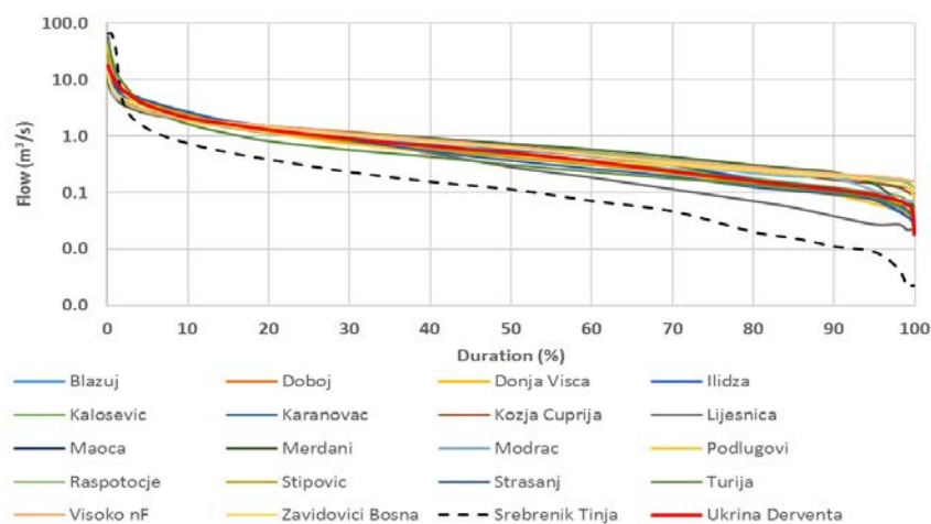
Figure 12. Relative flow duration curves (to mean flow) for the sub-catchments of Bosna River Basin that are similar to ungauged basins of Ukrina, Tinja and Brka
