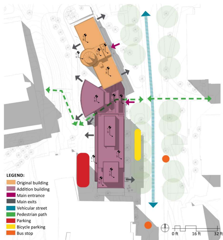
Figure 11. Site plan of the analyzed building (Source: Author [12]).
